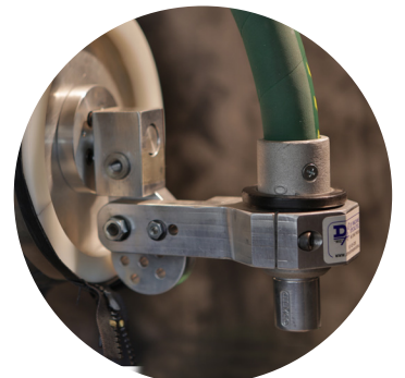
Robotic Blast Head
