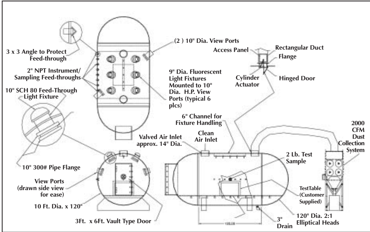
Explosive Test Cell
