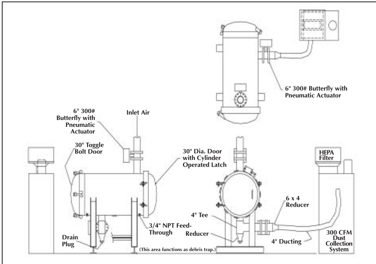
General Assembly 30 Inch Test Cell
